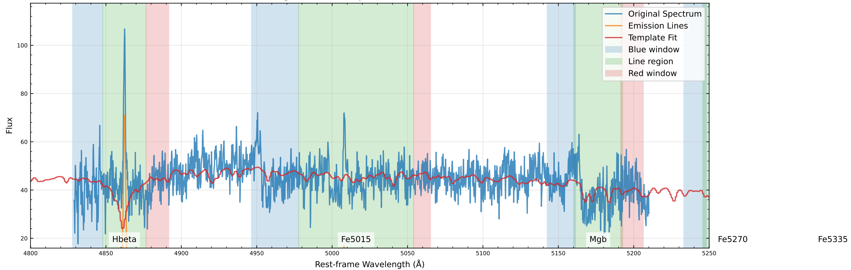
Original Data Comparison (v=-54.5 km/s)
