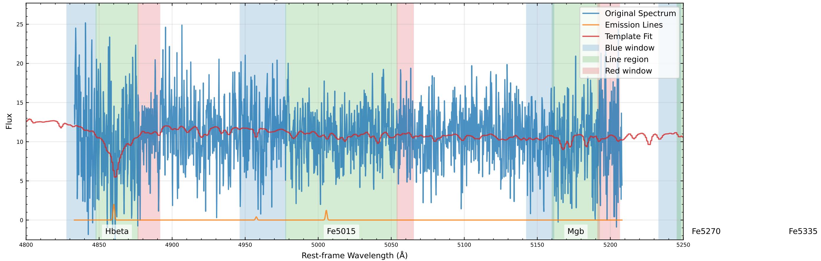
Original Data Comparison (v=-7.1 km/s)
