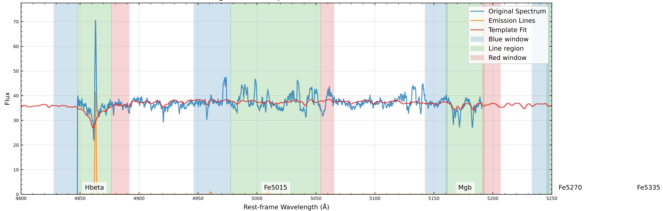
Original Data Comparison (v=-28.7 km/s)
