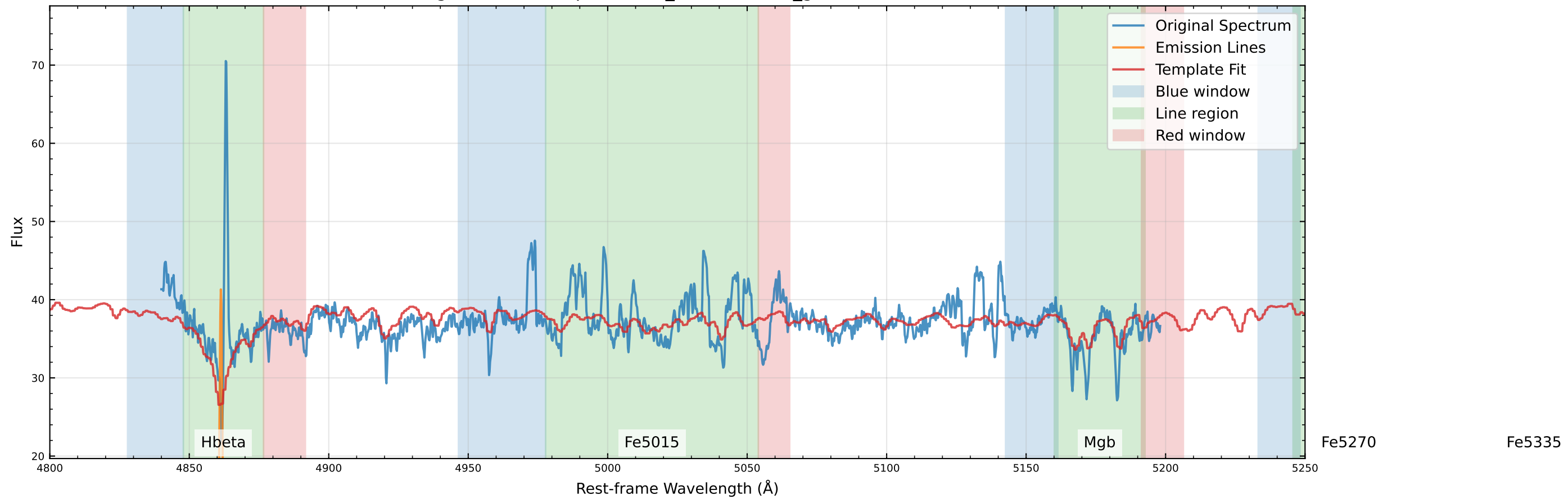
Original Data Comparison (v_star=-30.7, v_gas=83.1 km/s)
