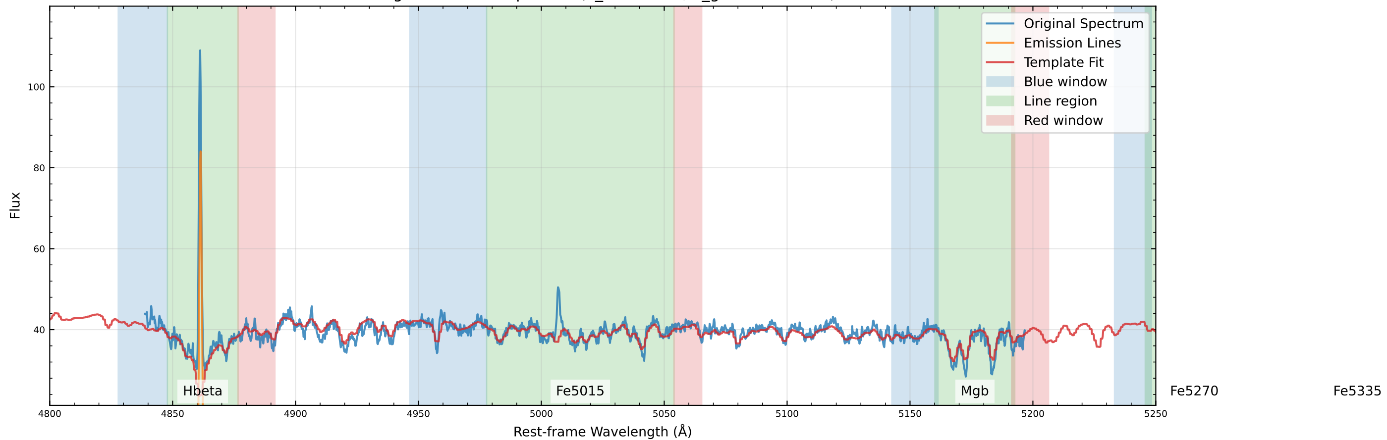
Original Data Comparison (v_star=41.3, v_gas=31.7 km/s)
