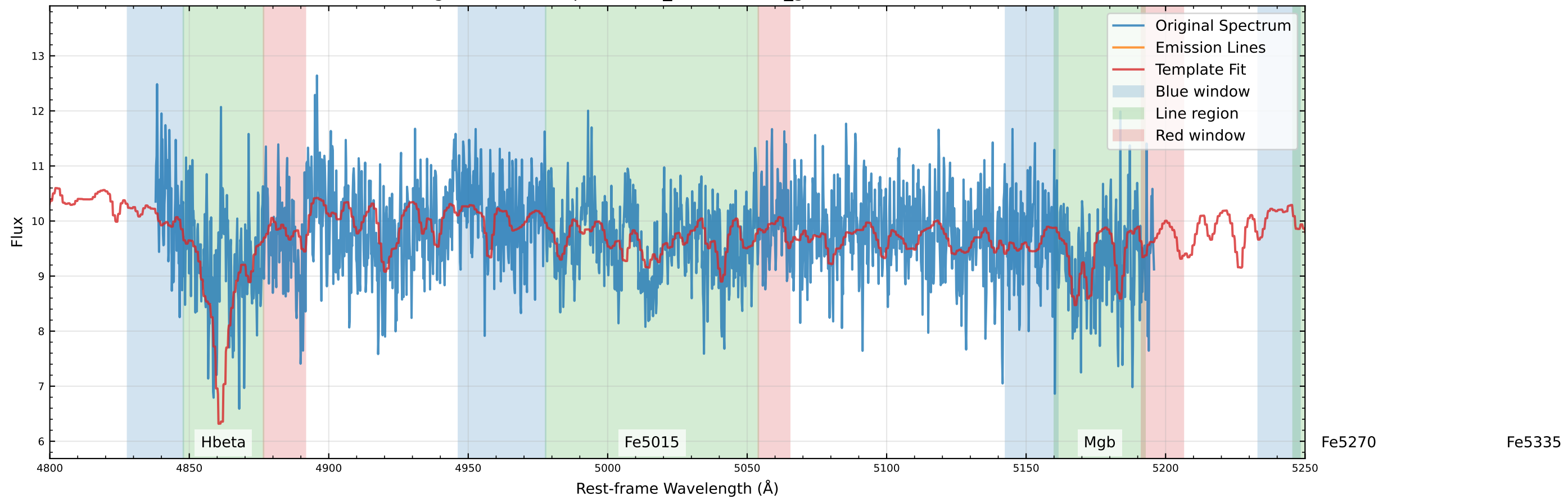
Original Data Comparison (v_star=96.4, v_gas=140.6 km/s)
