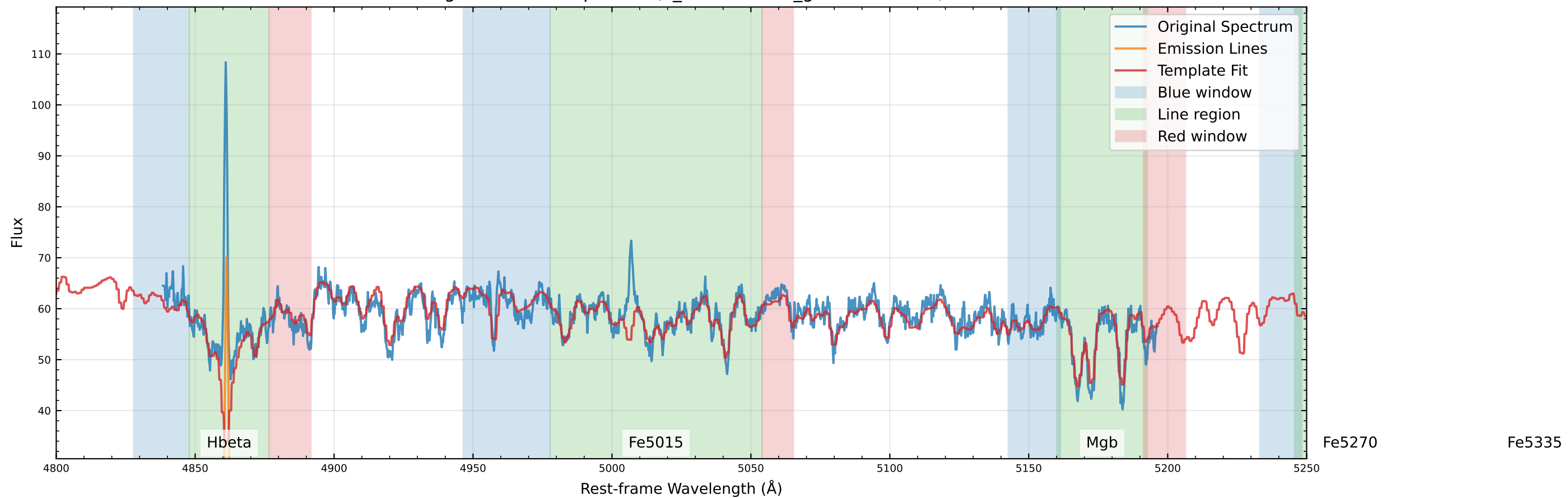
Original Data Comparison (v_star=64.3, v_gas=46.3 km/s)
