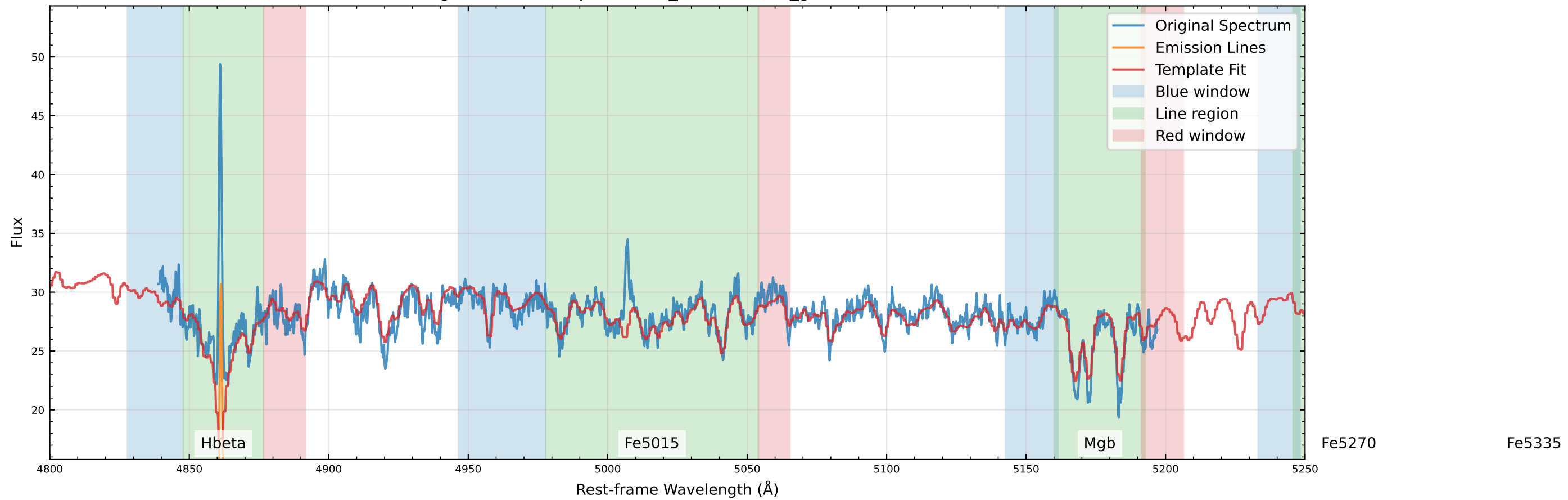
Original Data Comparison (v_star=30.6, v_gas=18.6 km/s)
