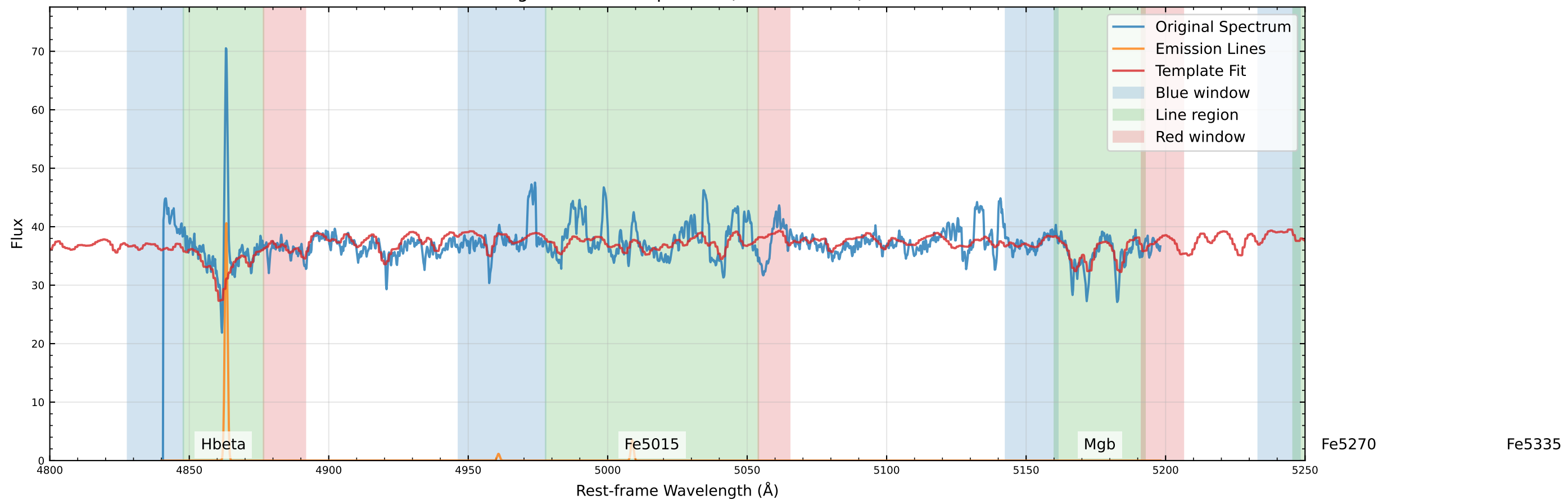
Original Data Comparison (v=-33.7 km/s)
