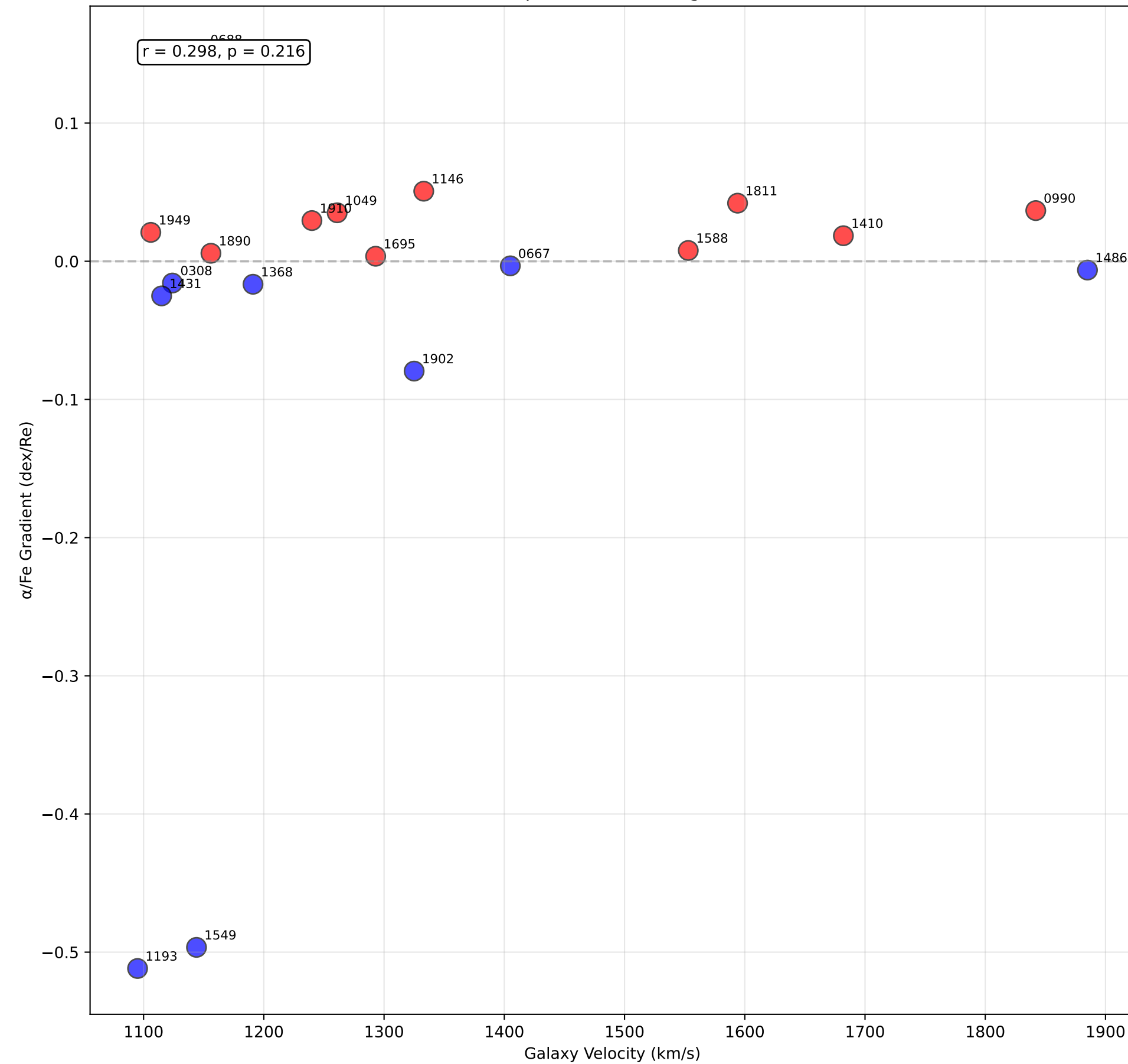
\alpha/\text{Fe} Gradient vs Galaxy Velocity (Red: positive, Blue: negative)
