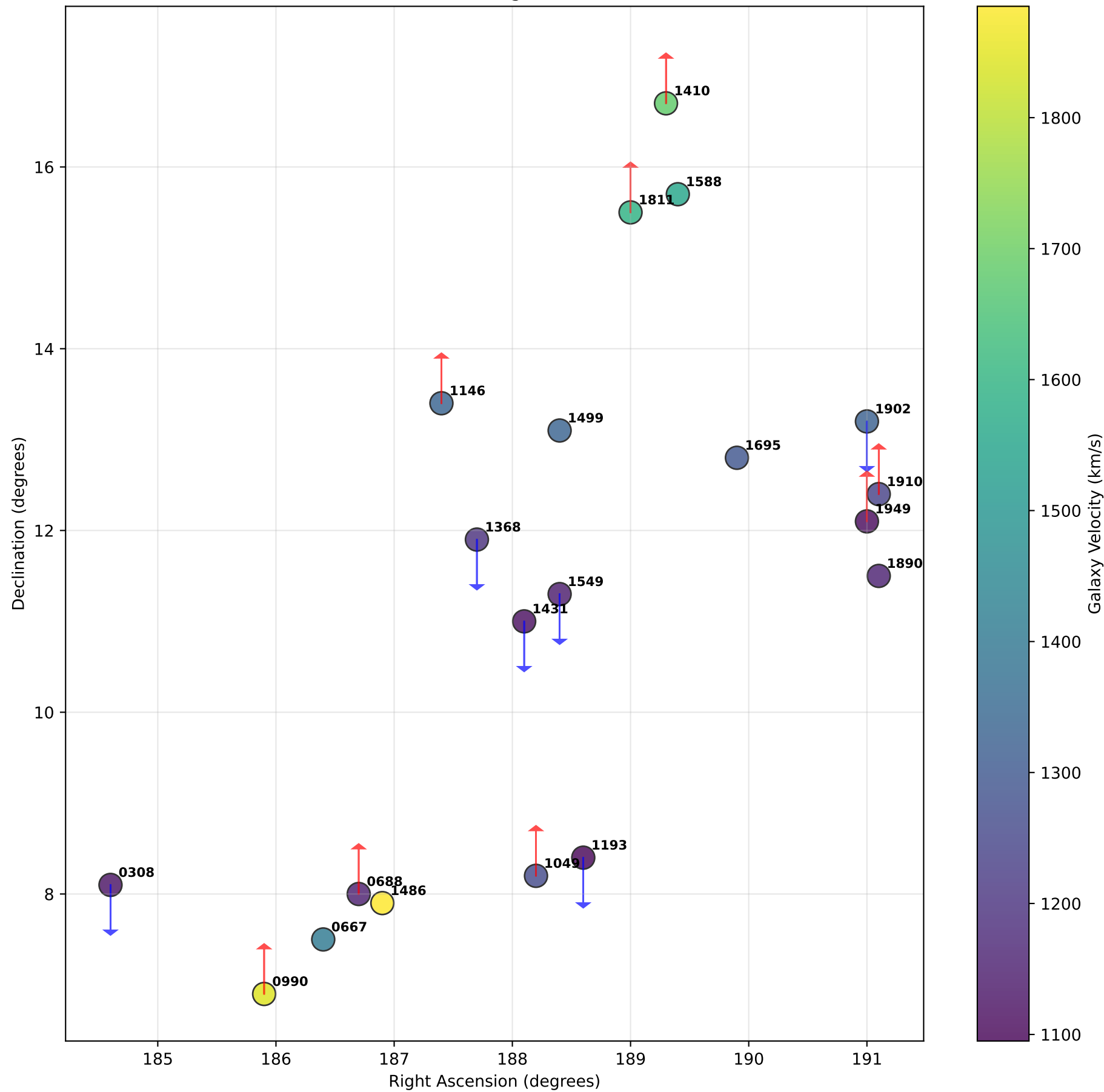
Virgo Cluster Galaxies - Velocity Color-Coded (Arrows indicate \alpha/\text{Fe} gradient direction)
