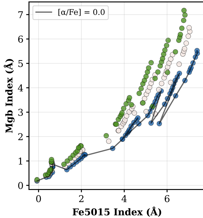
(a) Fe5015 vs Mgb
