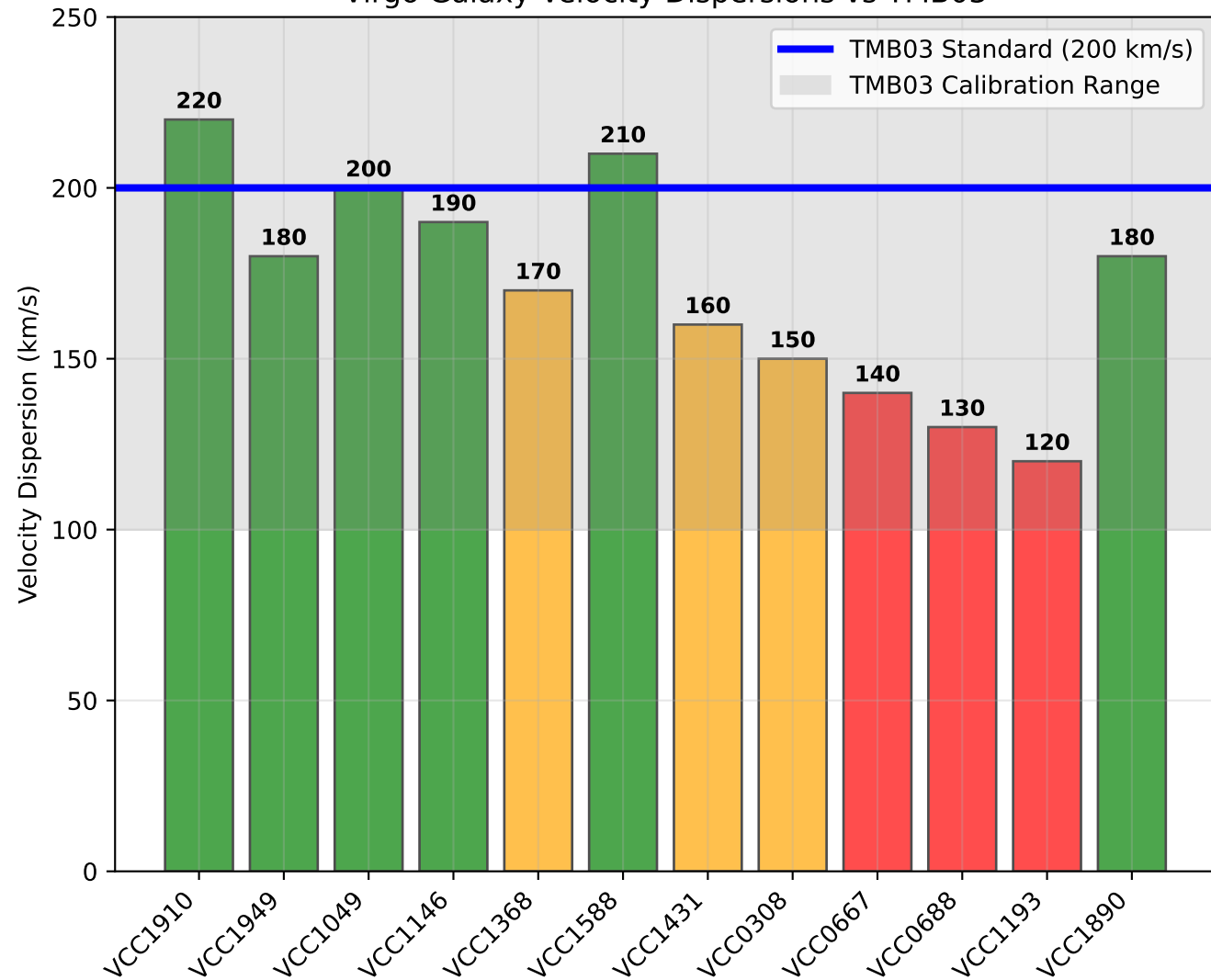
Virgo Galaxy Velocity Dispersions vs TMB03
