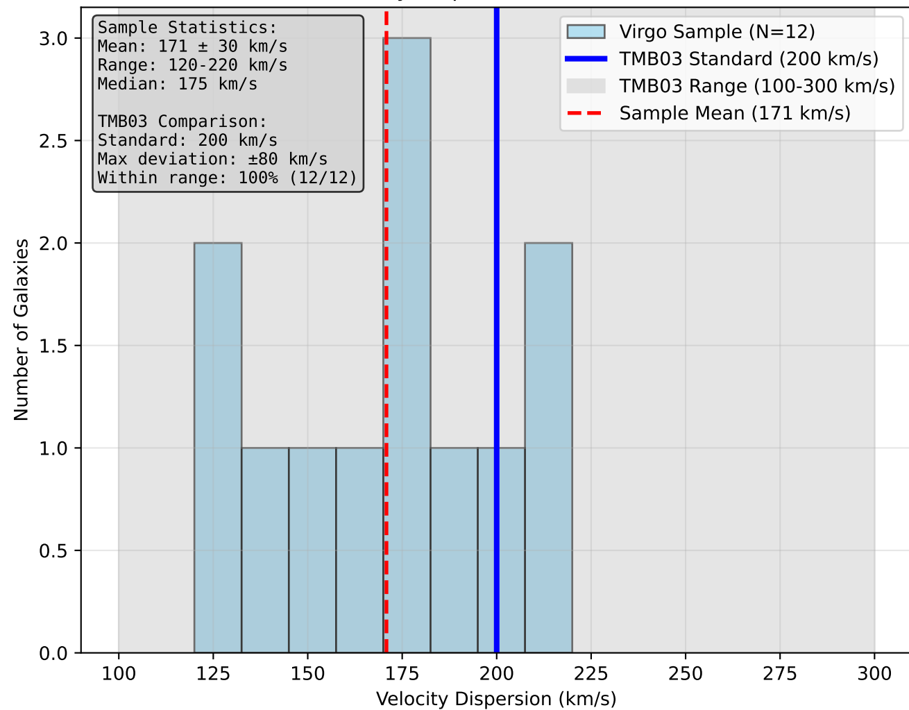
Velocity Dispersion Distribution
