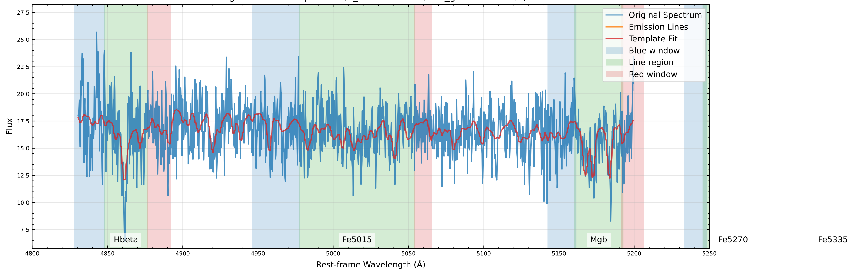
Original Data Comparison (v_star=25.8 km/s, v_gas=19.4 km/s)
