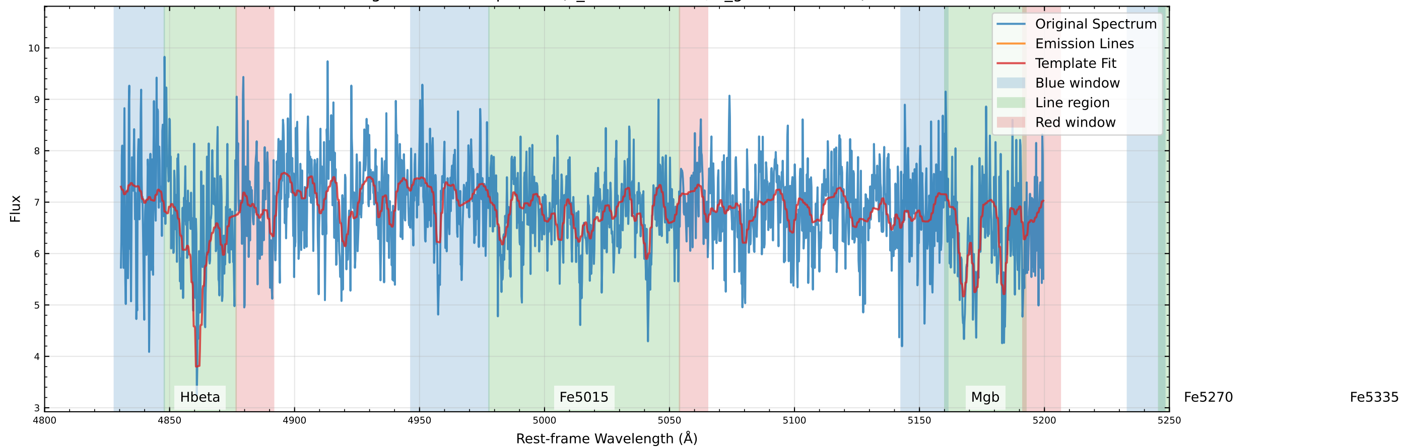
Original Data Comparison (v_star=-0.4 km/s, v_gas=-25.7 km/s)
