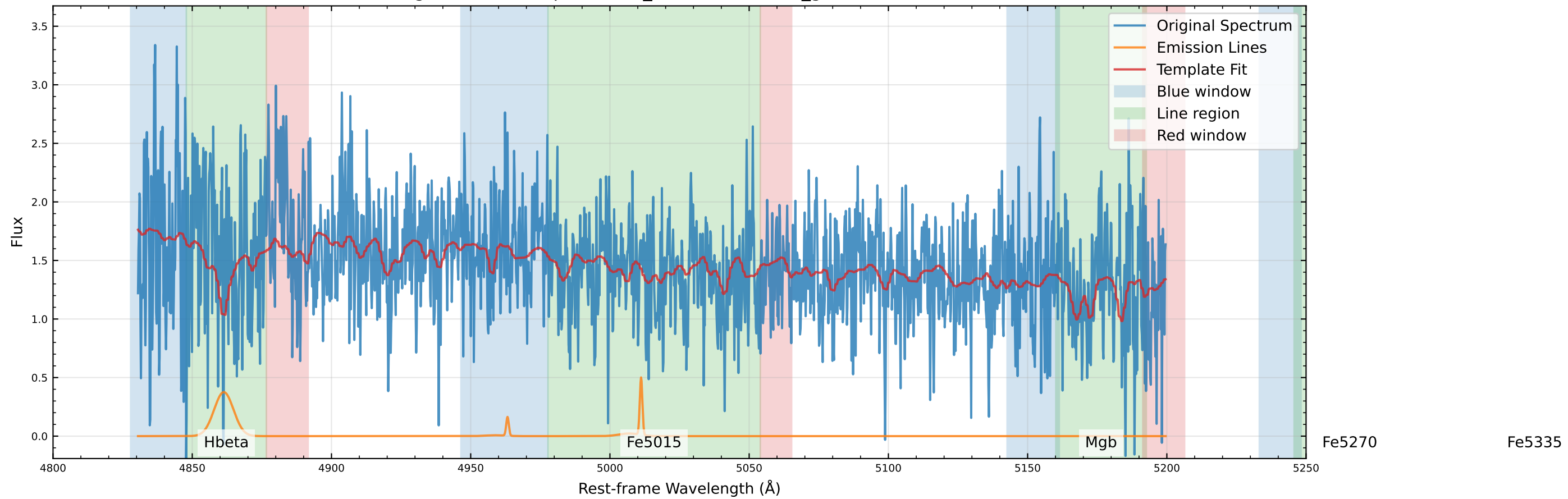
Original Data Comparison (v_star=6.6 km/s, v_gas=-261.0 km/s)
