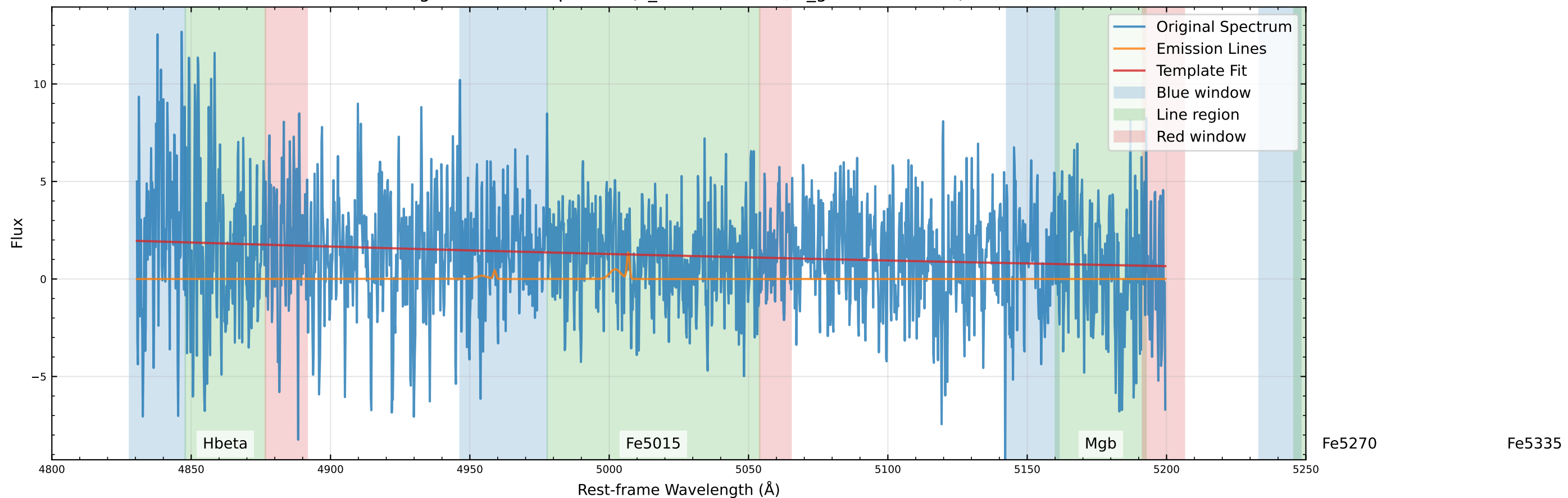
Original Data Comparison (v_star=0.0 km/s, v_gas=-19.9 km/s)
