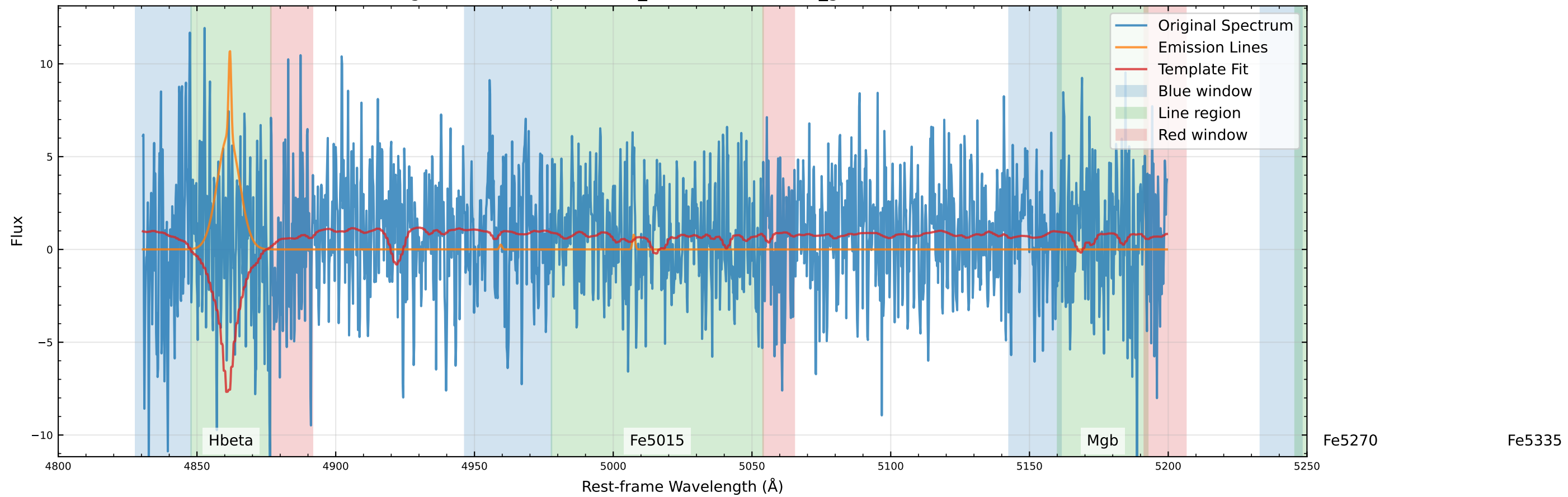
Original Data Comparison ( v_{\text{star}}=398.4 km/s, v_{\text{gas}}=430.1 km/s)
