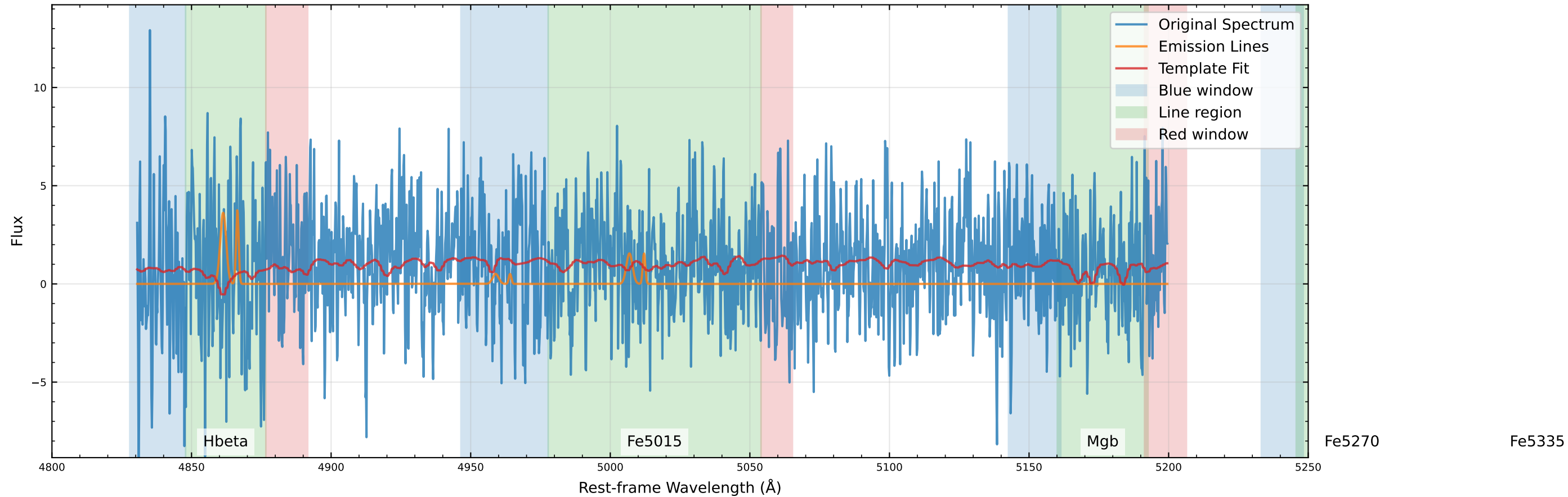
Original Data Comparison (v_star=-357.0 km/s, v_gas=-657.0 km/s)
