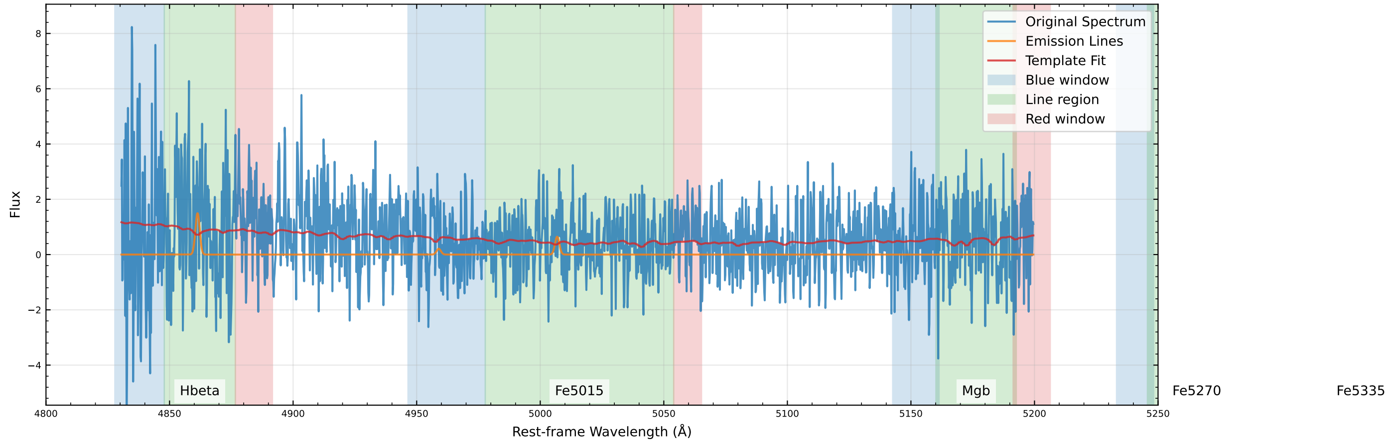
Original Data Comparison (v_star=38.6 km/s, v_gas=46.9 km/s)
