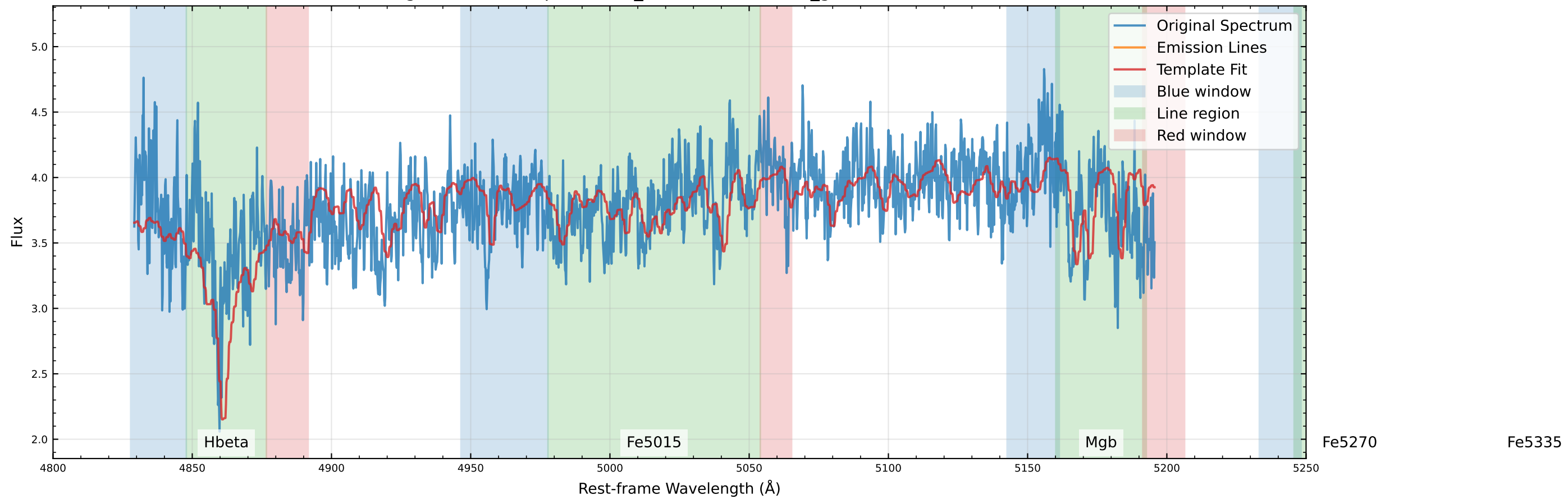
Original Data Comparison (v_star=-98.8 km/s, v_gas=-373.9 km/s)
