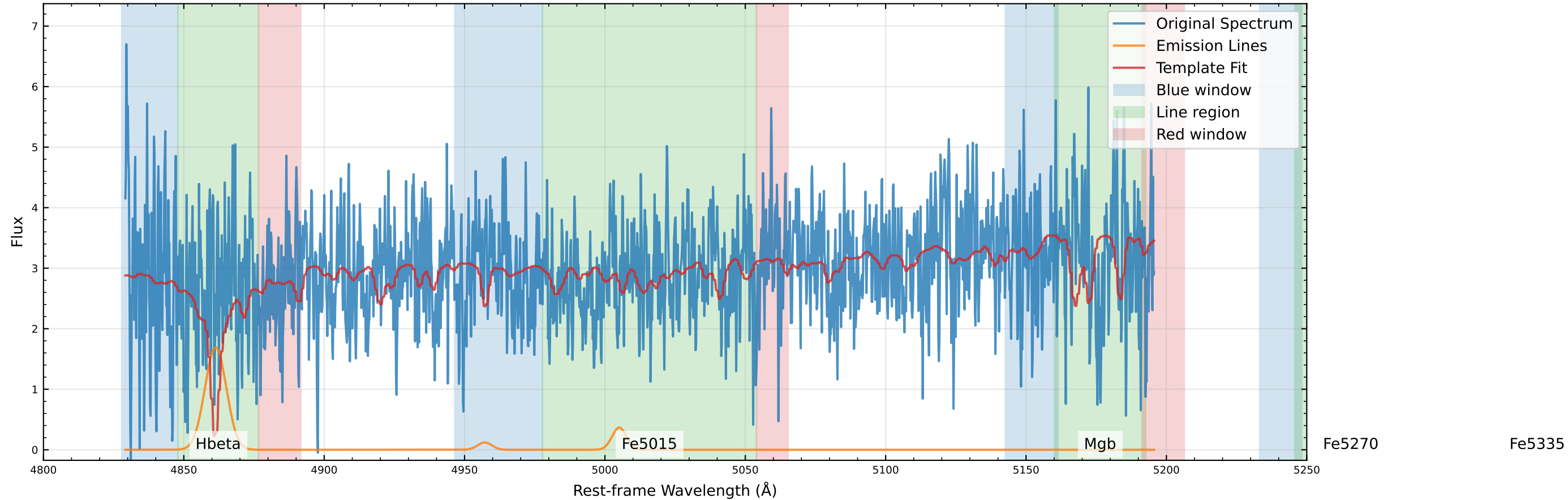
Original Data Comparison (v_star=303.8 km/s, v_gas=297.8 km/s)
