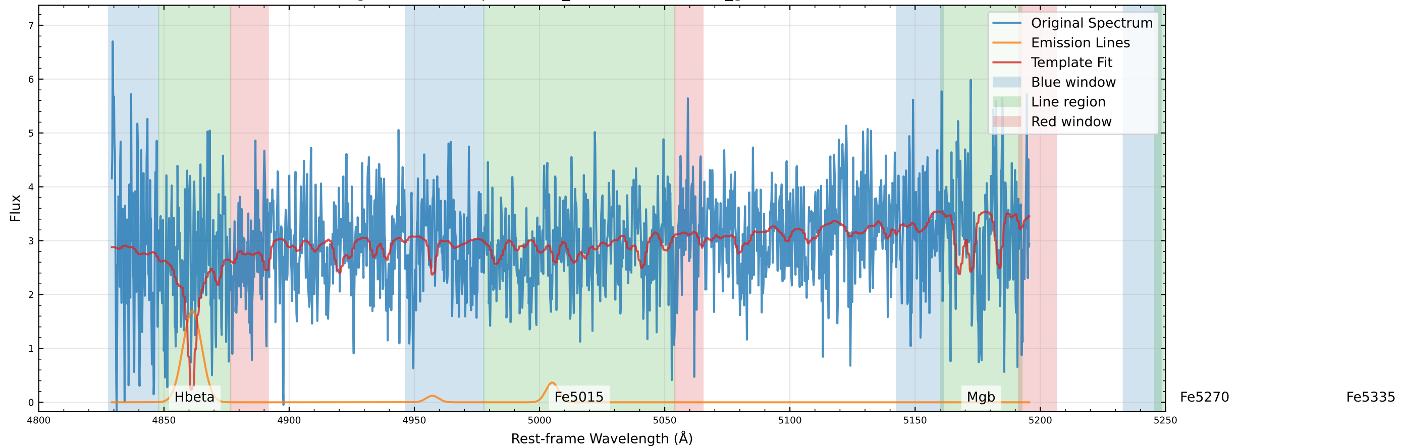
Original Data Comparison (v_star=303.8 km/s, v_gas=297.8 km/s)
