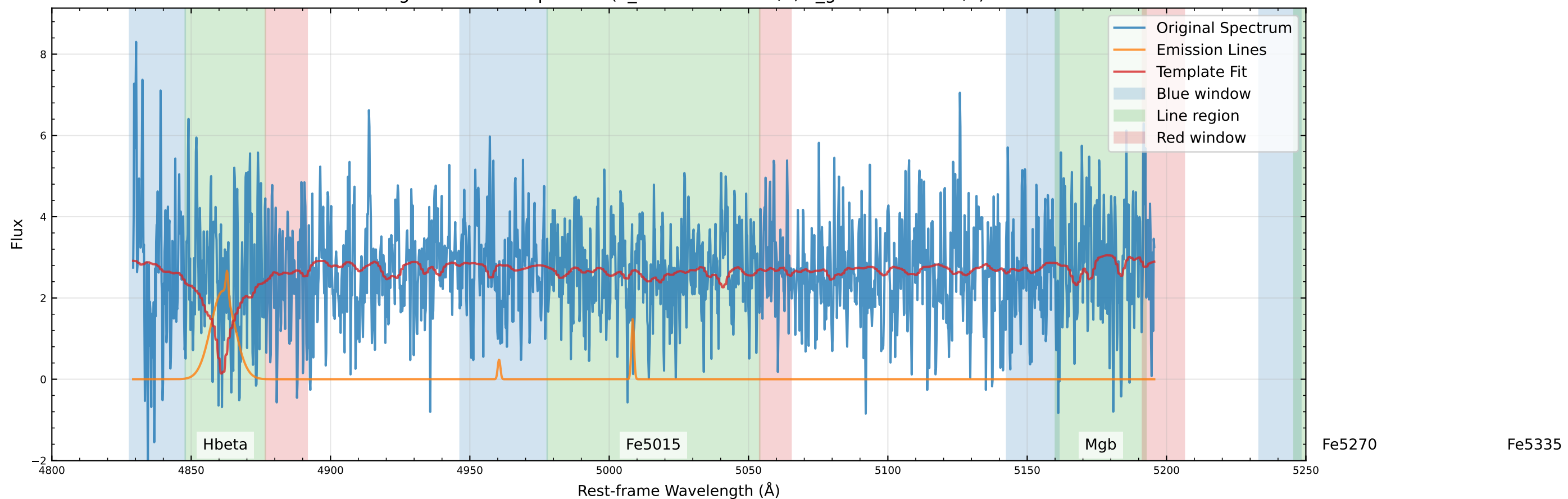
Original Data Comparison (v_star=-362.9 km/s, v_gas=-438.7 km/s)
