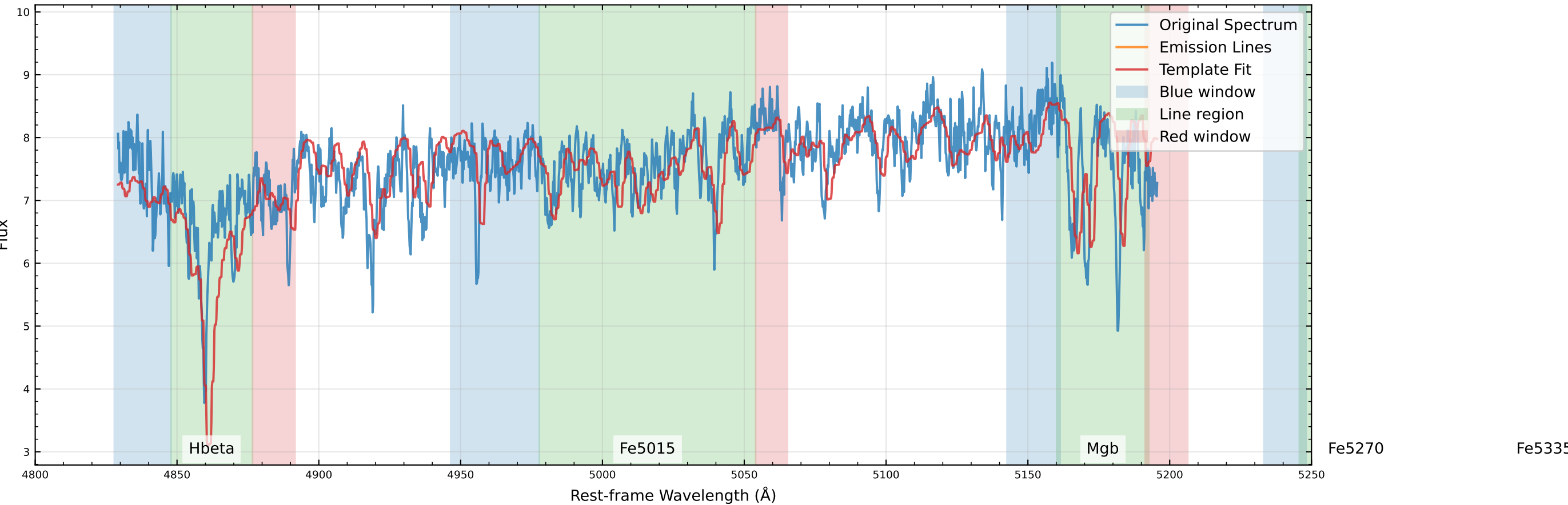
Original Data Comparison (v_star=-100.8 km/s, v_gas=-99.1 km/s)
