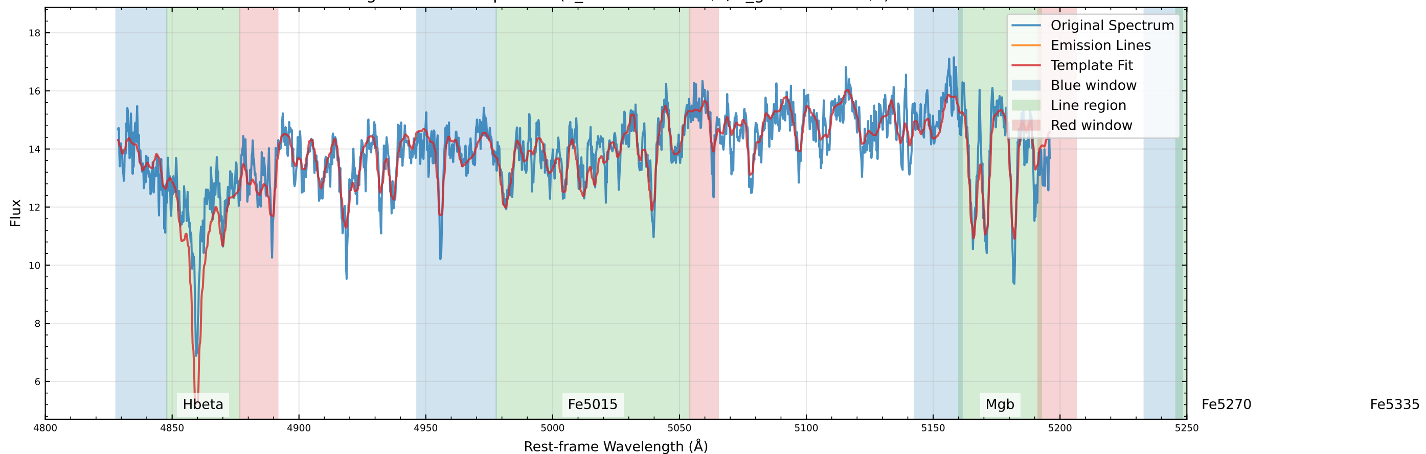
Original Data Comparison (v_star=-101.8 km/s, v_gas=-77.4 km/s)
