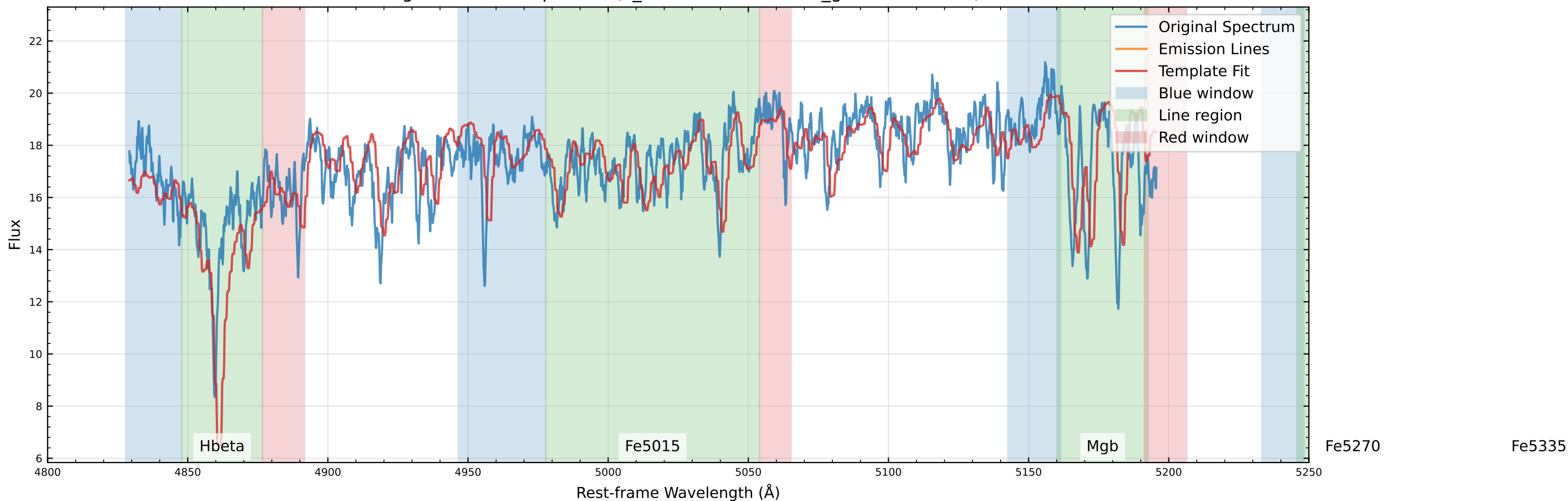
Original Data Comparison (v_star=-101.8 km/s, v_gas=-45.7 km/s)
