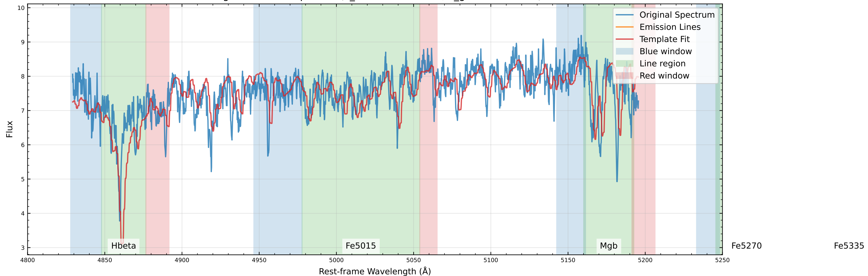
Original Data Comparison (v_star=-100.8 km/s, v_gas=-99.1 km/s)
