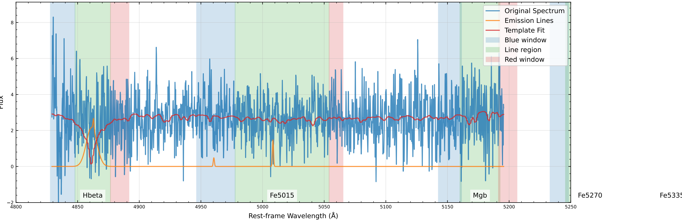
Original Data Comparison (v_star=-362.9 km/s, v_gas=-438.7 km/s)
