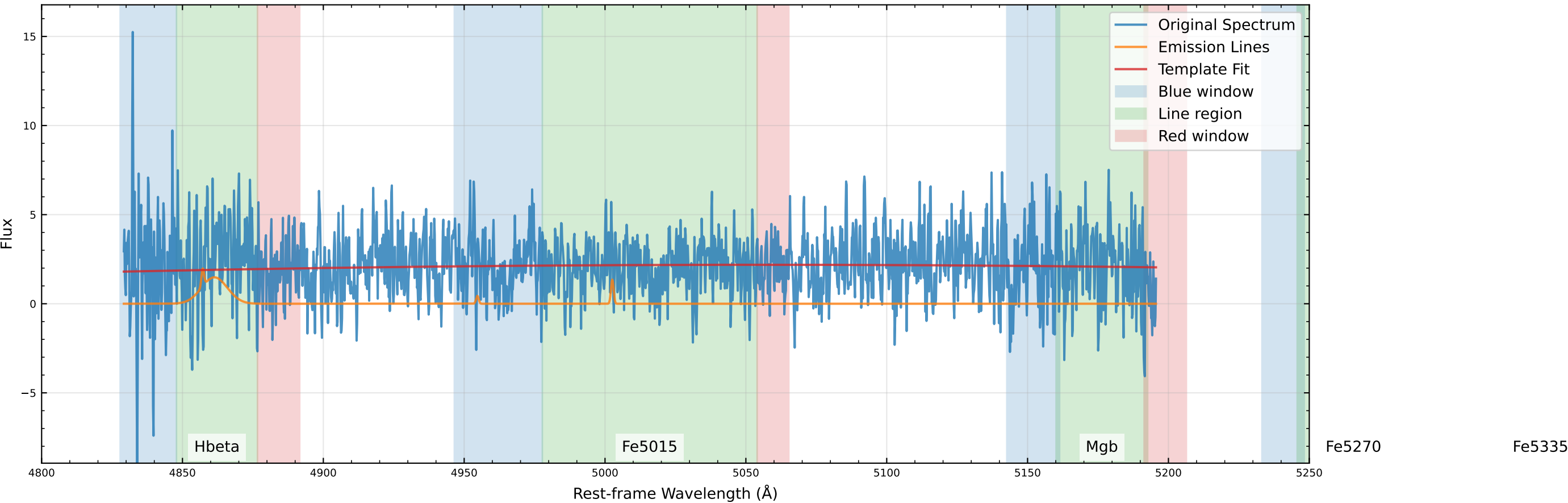
Original Data Comparison (v_star=0.0 km/s, v_gas=300.0 km/s)
