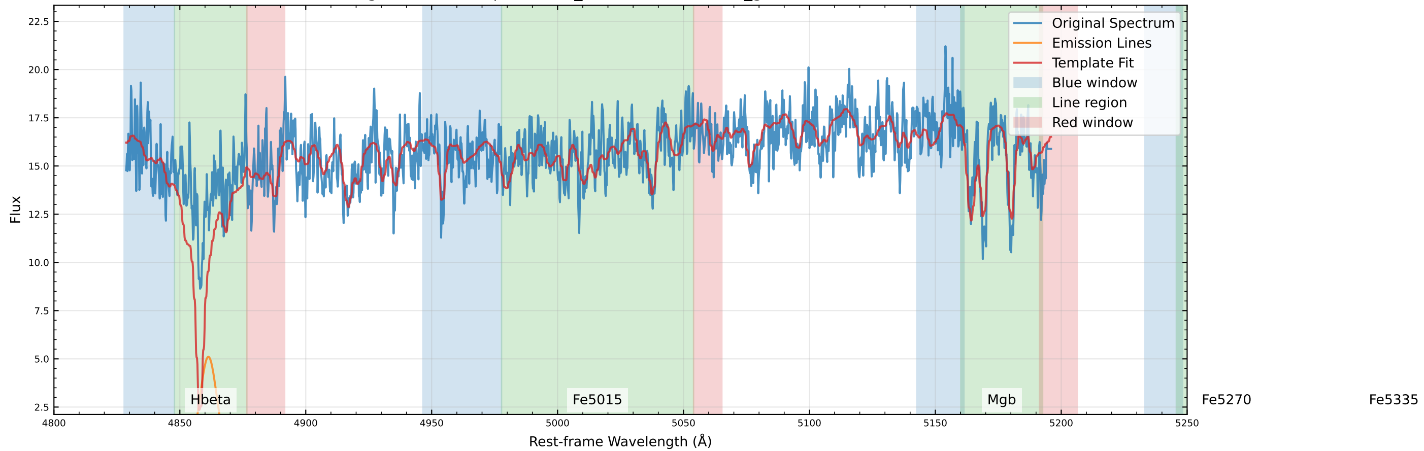
Original Data Comparison (v_star=-197.5 km/s, v_gas=-237.8 km/s)
