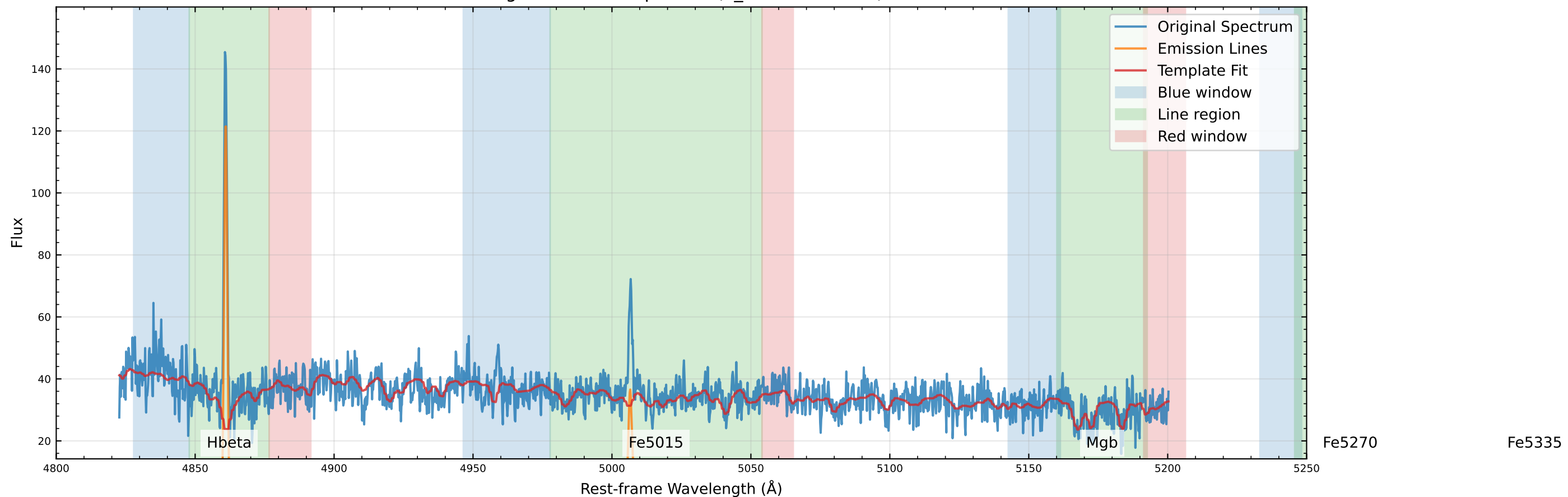
Original Data Comparison (v_star=-3.6 km/s)
