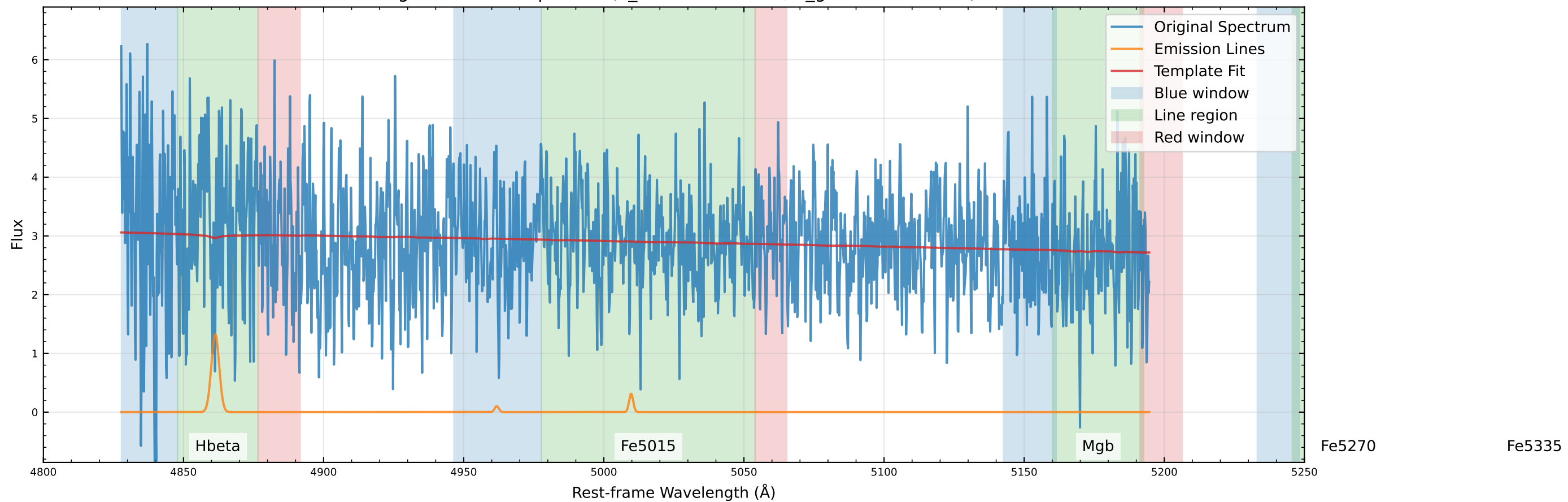
Original Data Comparison (v_star=-40.2 km/s, v_gas=-249.8 km/s)
