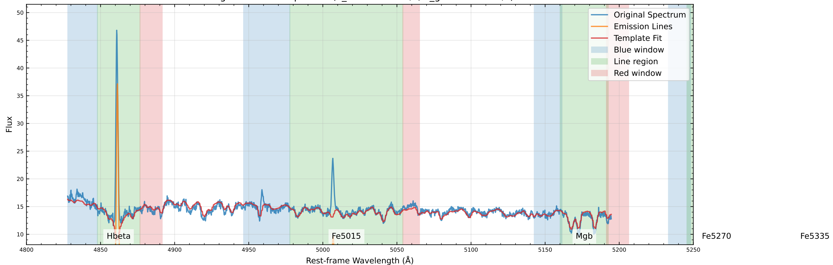
Original Data Comparison (v_star=-4.5 km/s, v_gas=-20.7 km/s)
