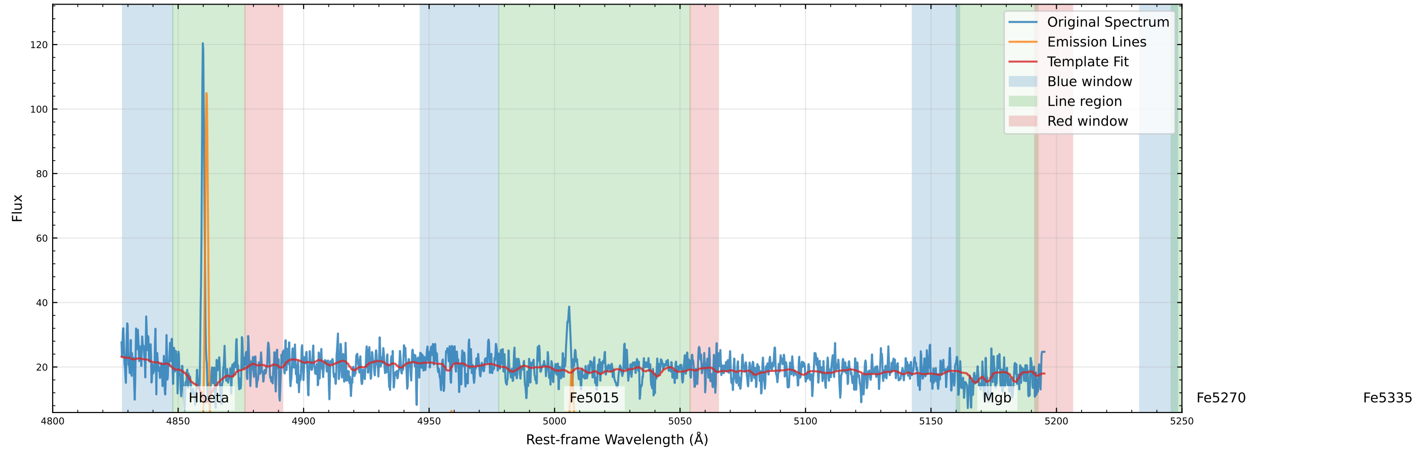
Original Data Comparison (v_star=-101.4 km/s, v_gas=-87.4 km/s)
