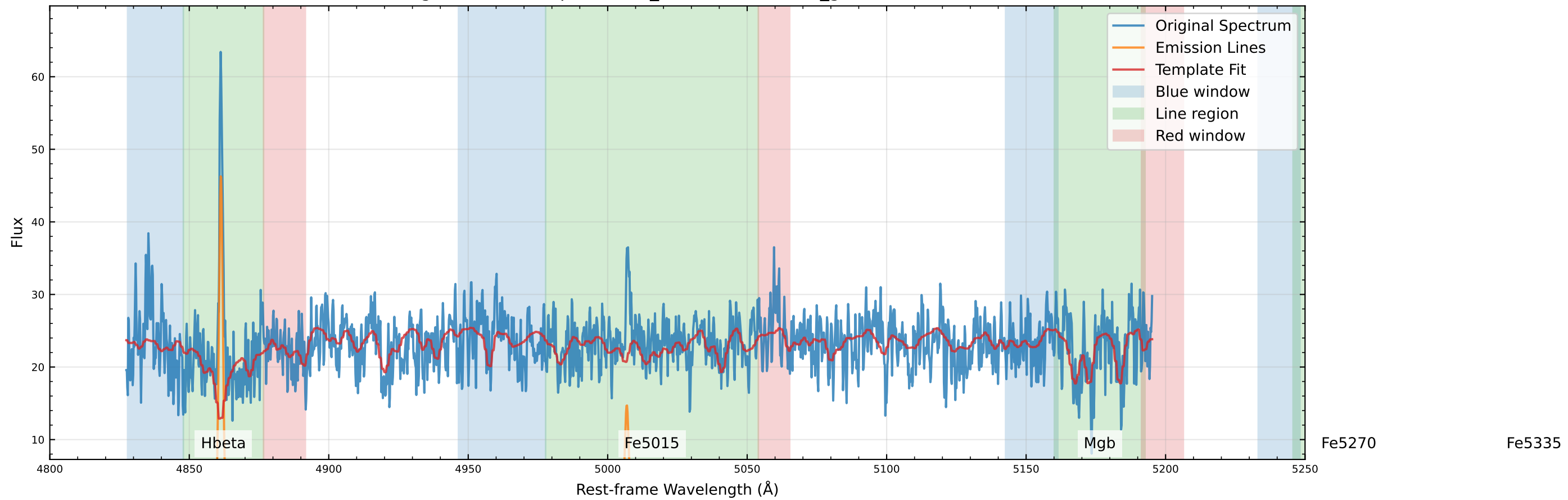
Original Data Comparison (v_star=35.6 km/s, v_gas=7.8 km/s)
