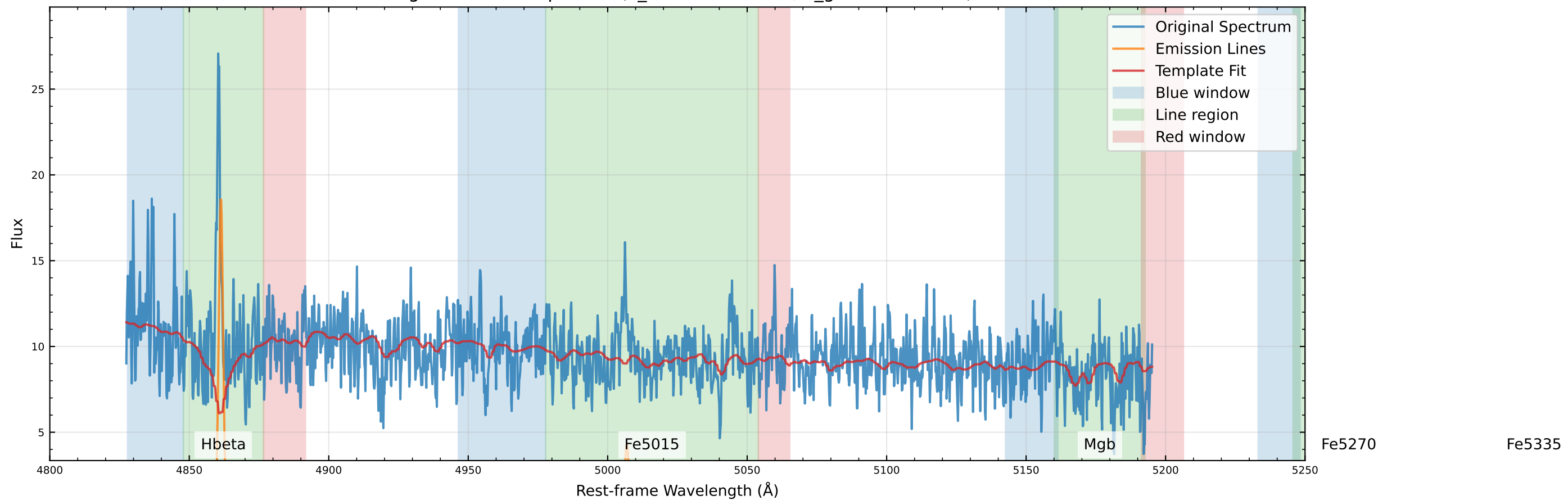
Original Data Comparison (v_star=-92.5 km/s, v_gas=-54.0 km/s)
