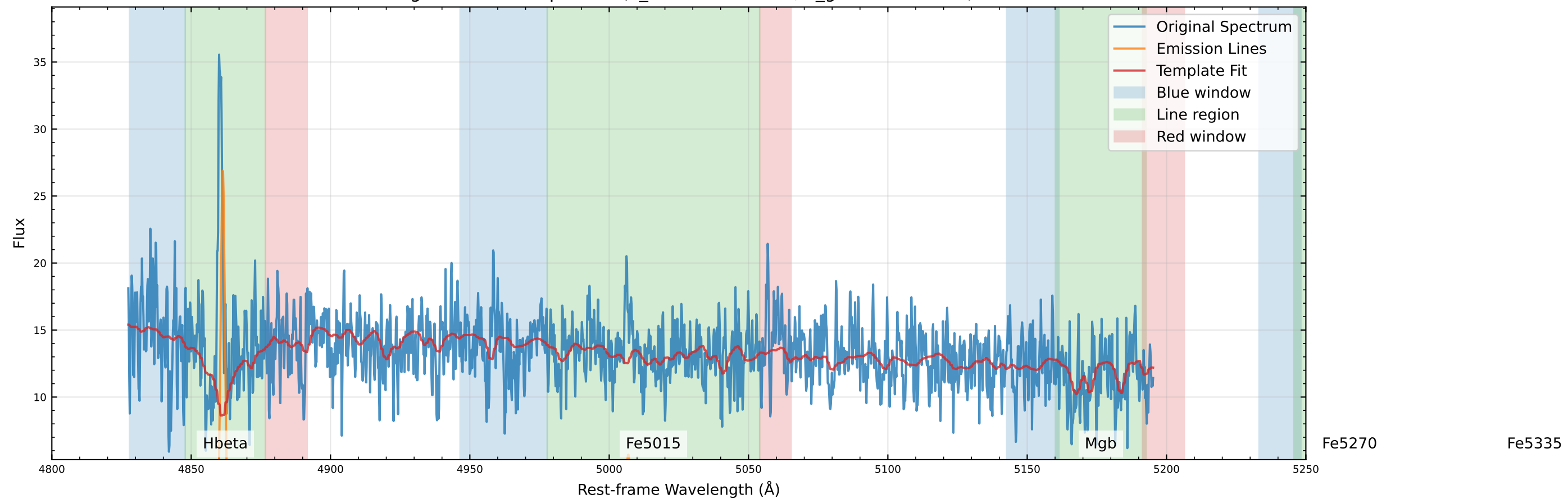
Original Data Comparison (v_star=-61.9 km/s, v_gas=-57.4 km/s)
