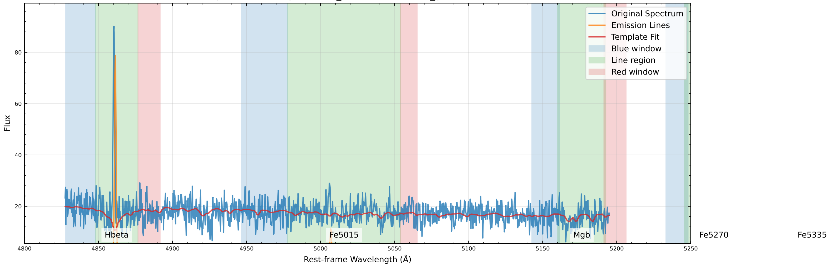
Original Data Comparison (v_star=-37.2 km/s, v_gas=-59.4 km/s)
