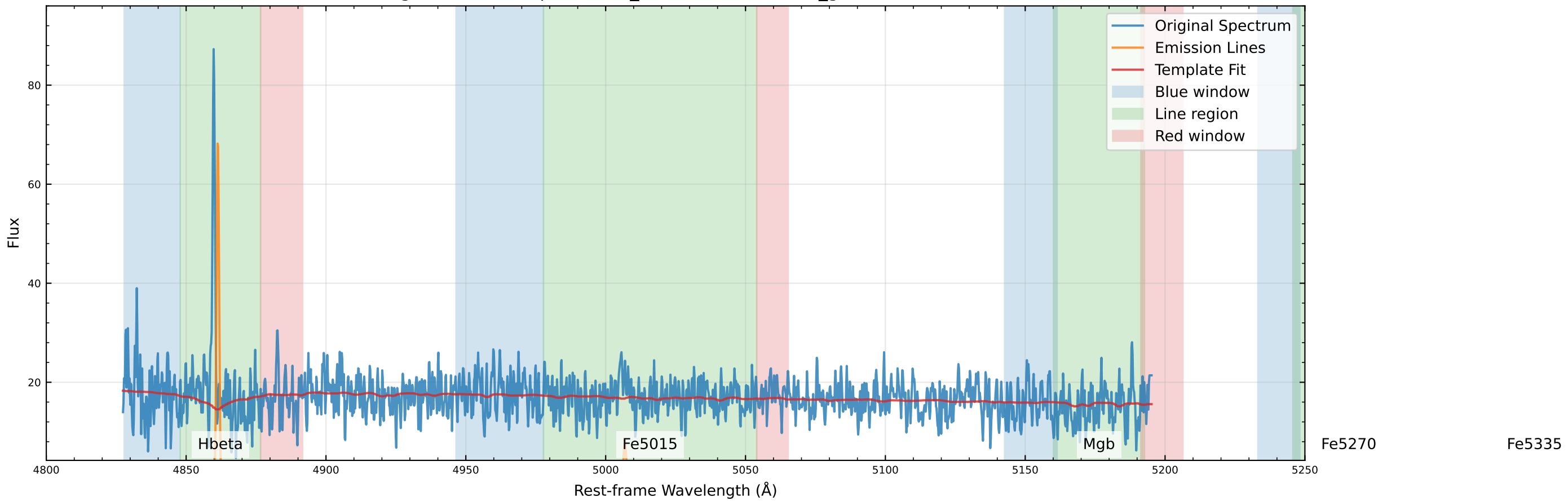
Original Data Comparison (v_star=-101.7 km/s, v_gas=-90.5 km/s)
