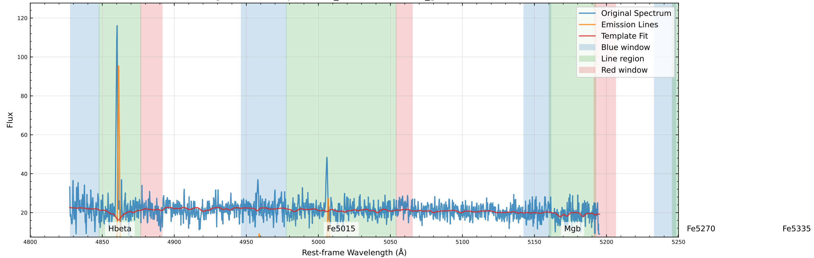
Original Data Comparison (v_star=-67.8 km/s, v_gas=-72.1 km/s)
