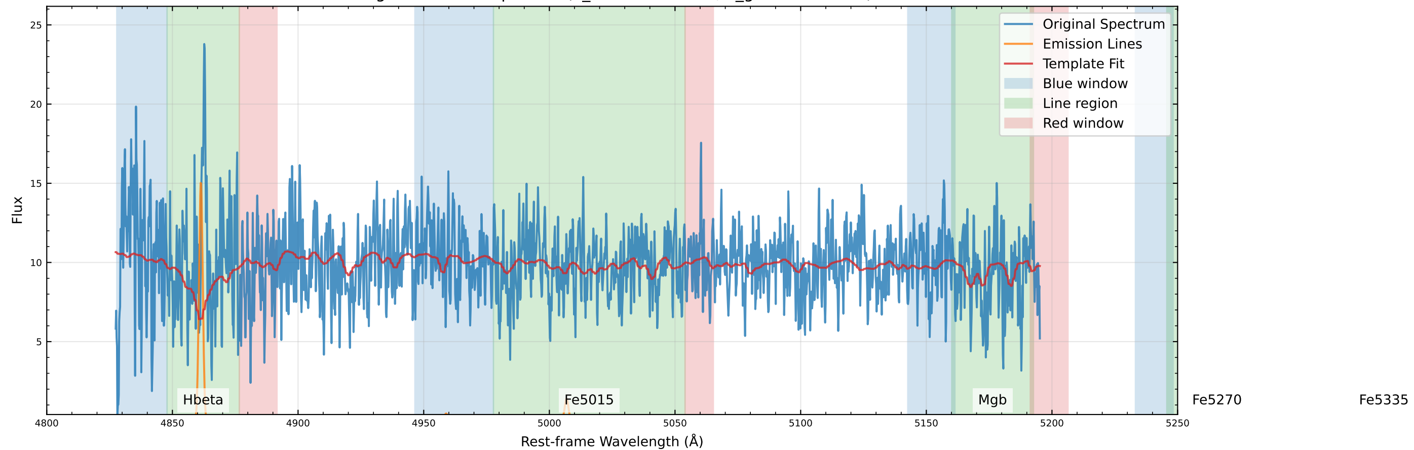
Original Data Comparison (v_star=98.7 km/s, v_gas=77.9 km/s)
