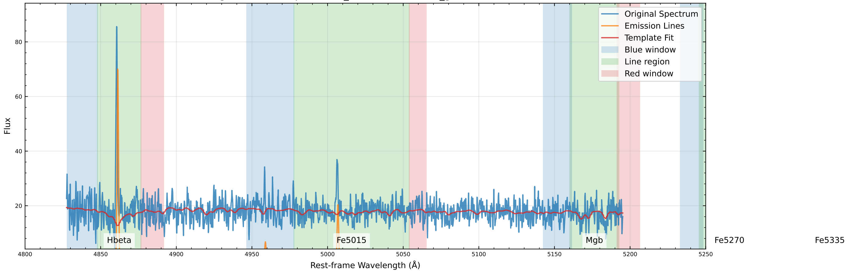
Original Data Comparison (v_star=-22.0 km/s, v_gas=-44.4 km/s)
