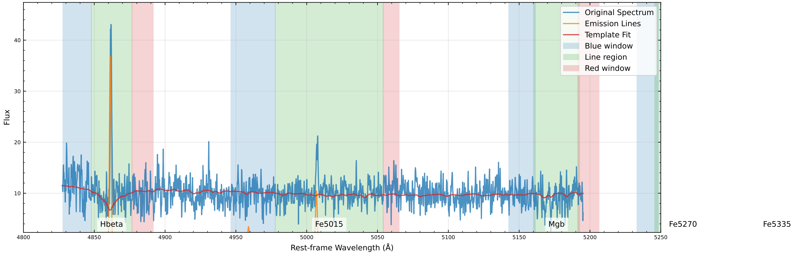
Original Data Comparison (v_star=31.8 km/s, v_gas=27.0 km/s)
