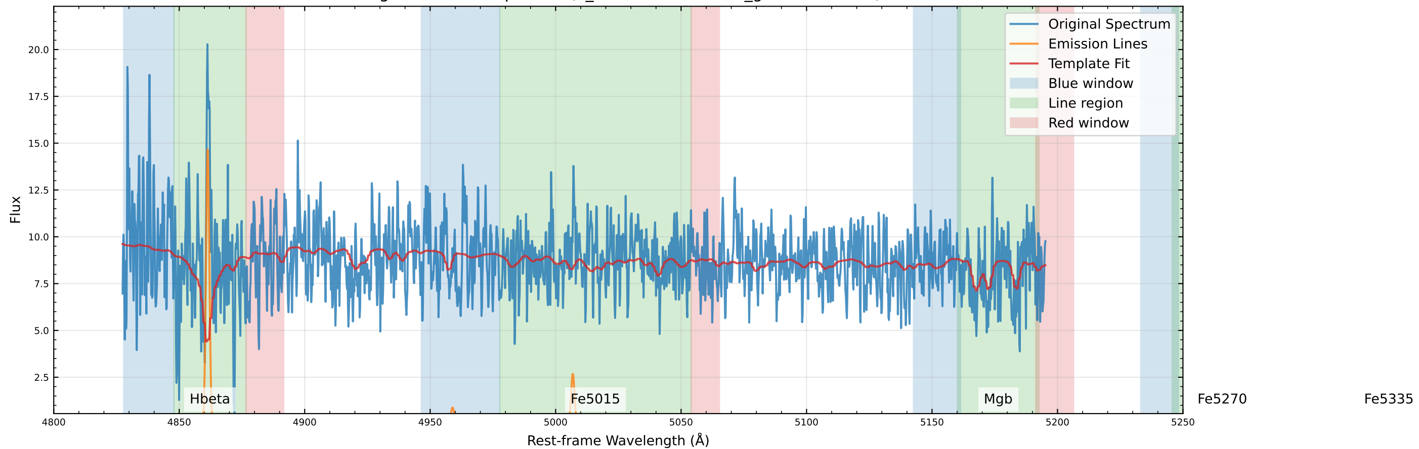
Original Data Comparison (v_star=-32.2 km/s, v_gas=13.8 km/s)
