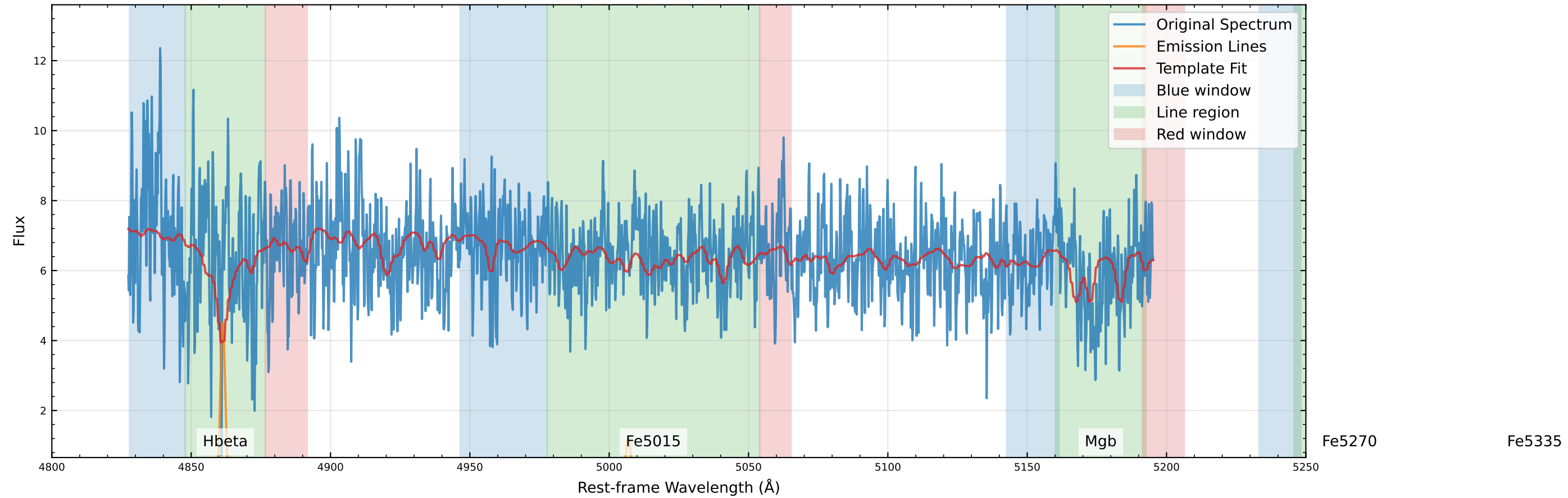
Original Data Comparison (v_star=100.8 km/s, v_gas=89.7 km/s)
