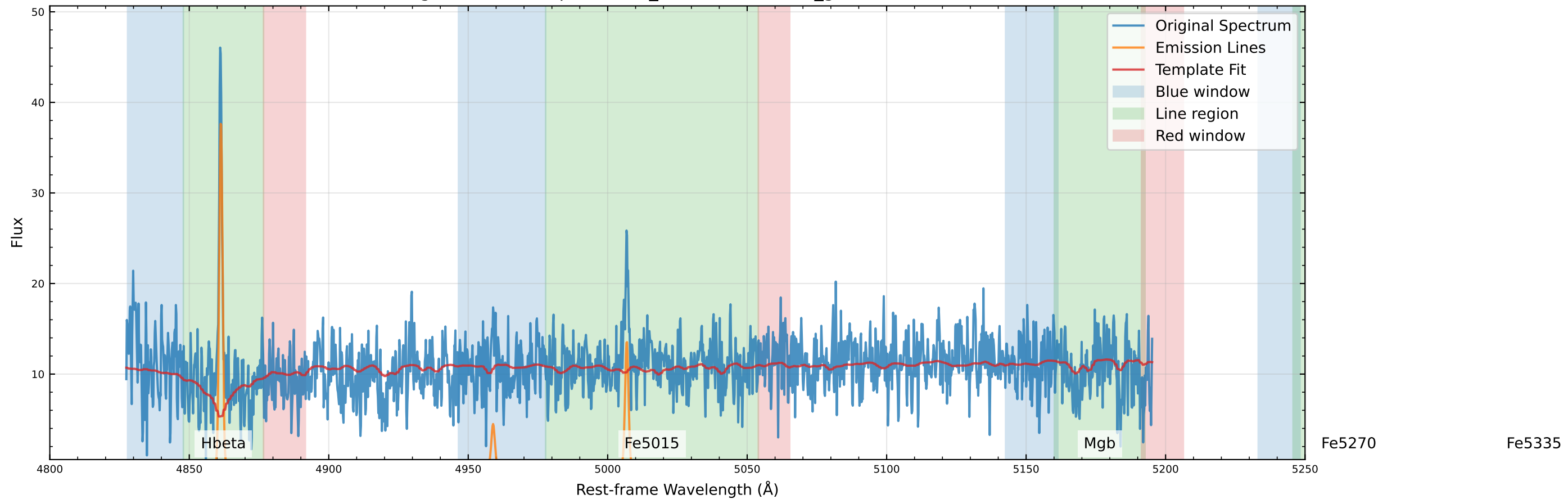
Original Data Comparison (v_star=-3.9 km/s, v_gas=-8.1 km/s)
