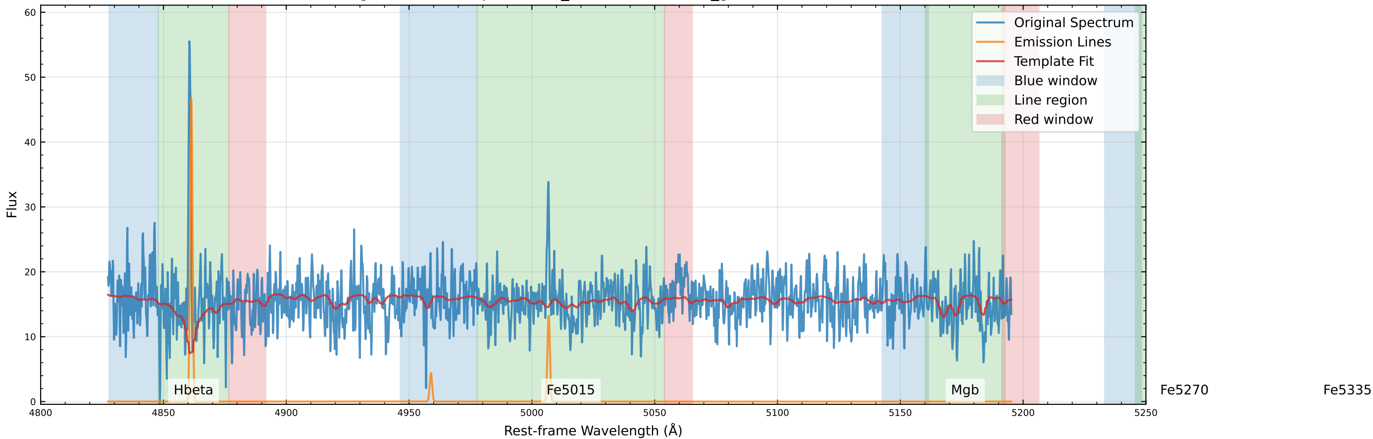
Original Data Comparison (v_star=12.2 km/s, v_gas=-37.3 km/s)
