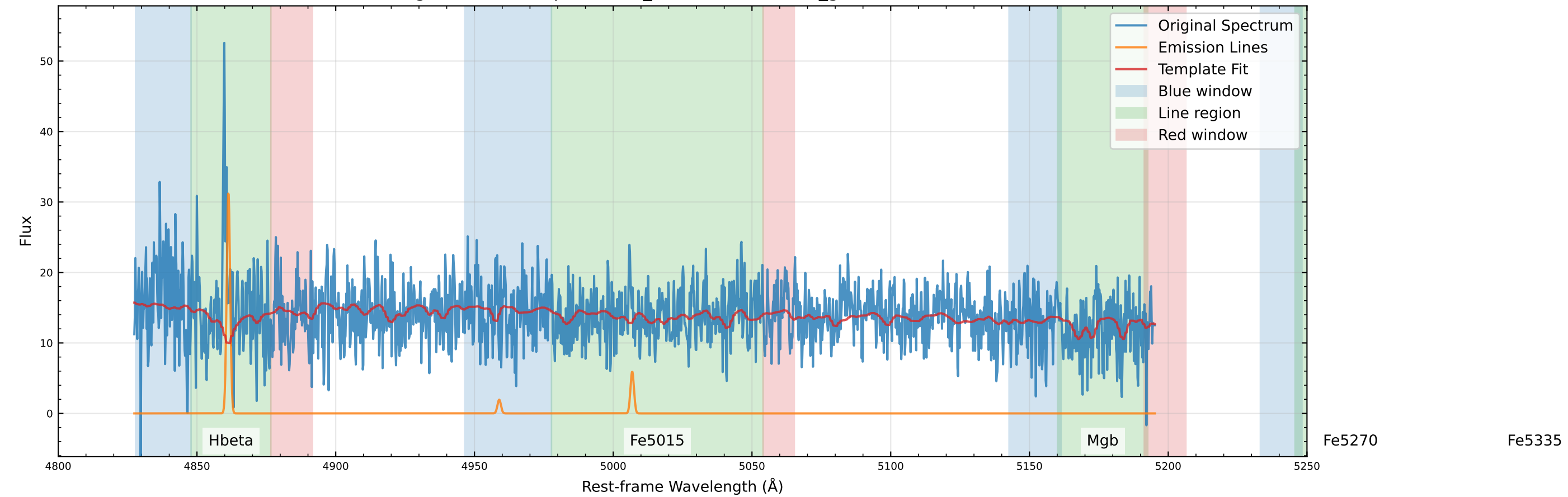
Original Data Comparison (v_star=-66.5 km/s, v_gas=-82.6 km/s)
