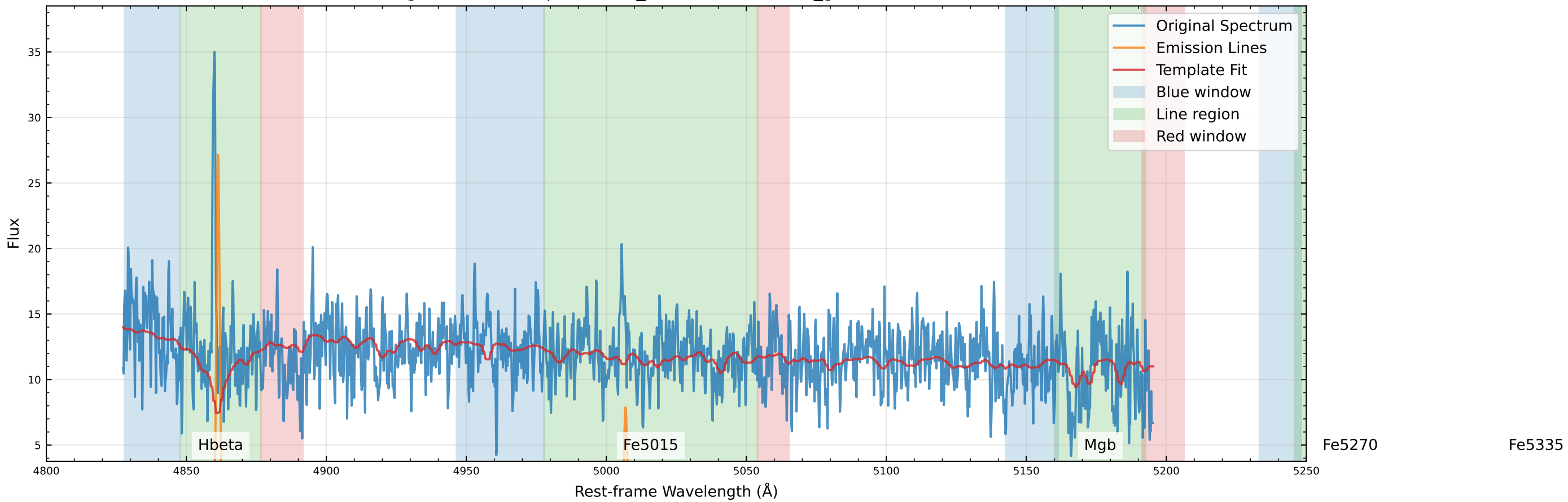
Original Data Comparison (v_star=-77.7 km/s, v_gas=-88.4 km/s)
