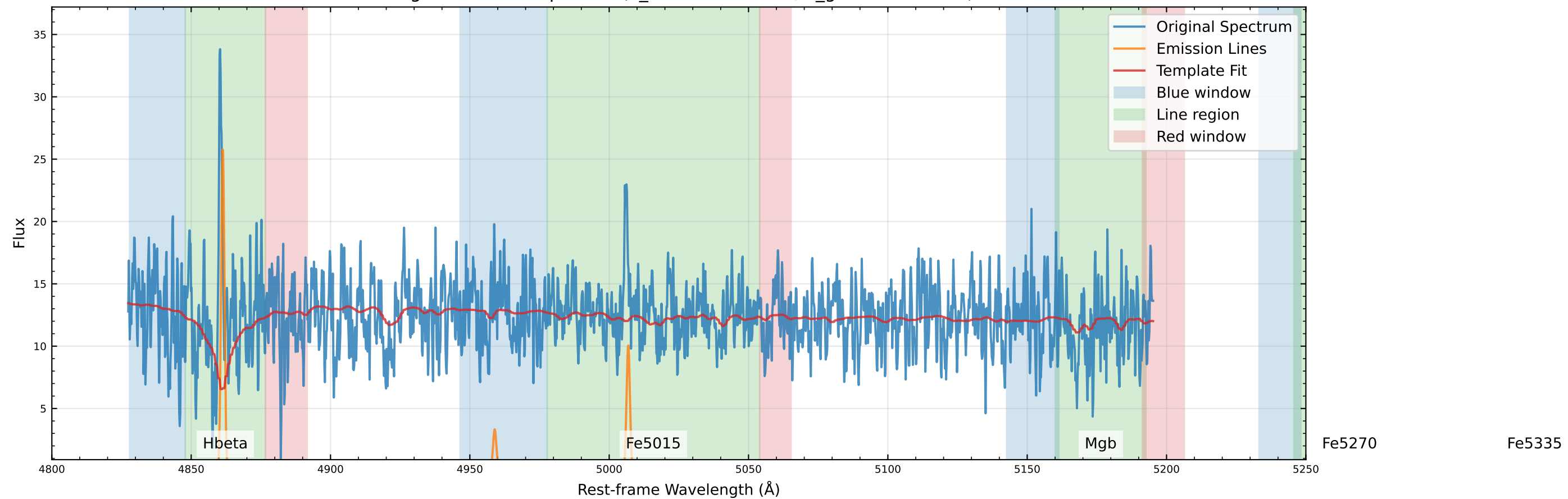
Original Data Comparison (v_star=-65.2 km/s, v_gas=-51.0 km/s)
